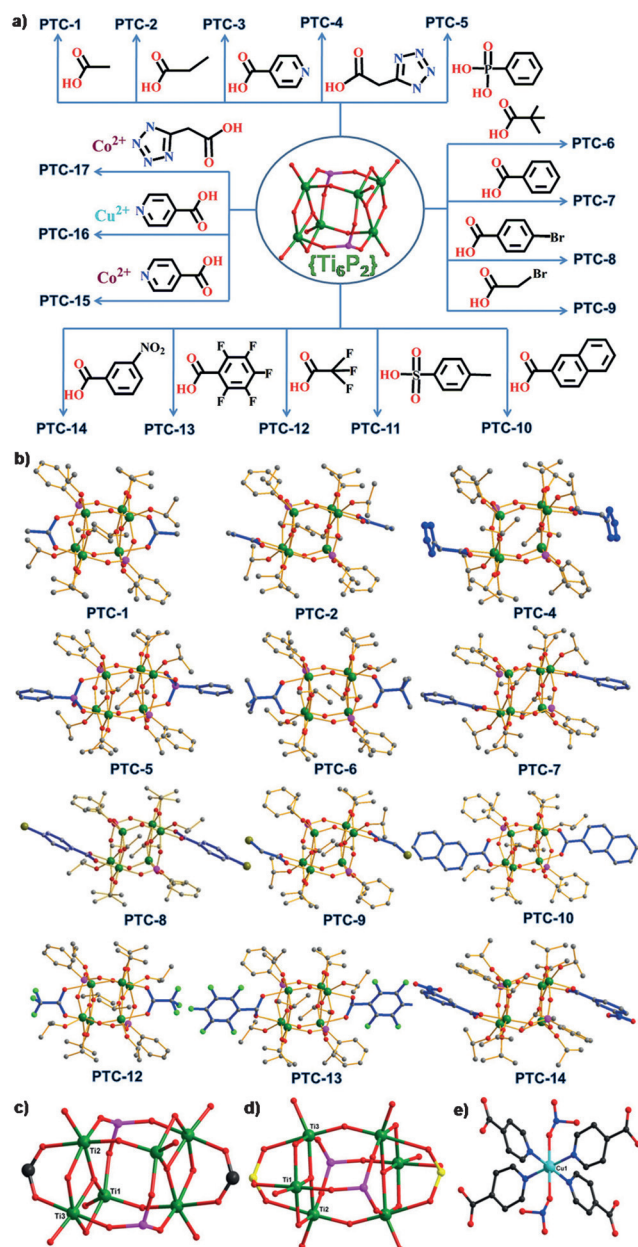
Figure 2. a) Illustration of the assembly of PTC-1-17 . b) Crystal structures of the {Ti 6 } cluster family, with the functionalized ligands highlighted in blue color. c,d) Representative coordination modes of {Ti 6 } in PTC-1 and PTC-11 . e) Coordination environment of the Cu ions in PTC-16 .
